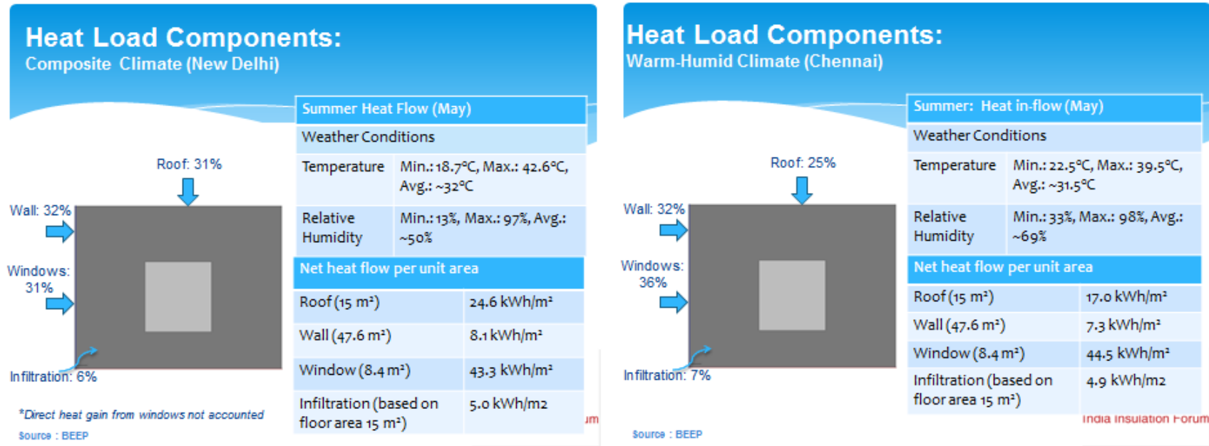
FIGURE 4 : EXAMPLES OF HEAT LOAD COMPONENTS IN DELHI AND CHENNAI IN SUMMER
