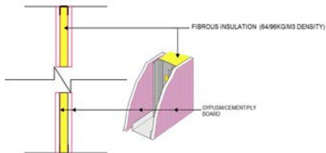
FIGURE 22: PARTITION WALL INSULATION
