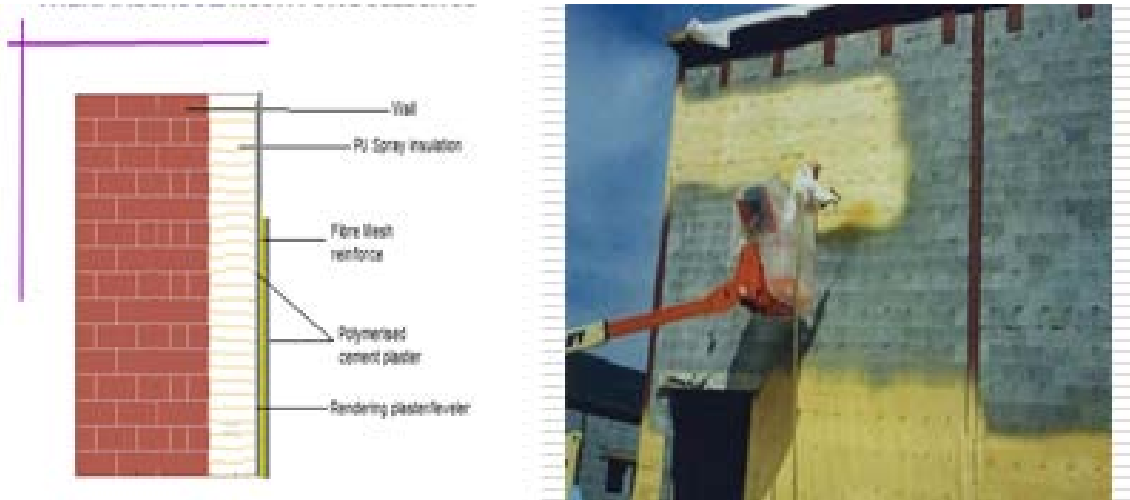
FIGURE 20: SPRAY CAST IN-SITU INSULATION
